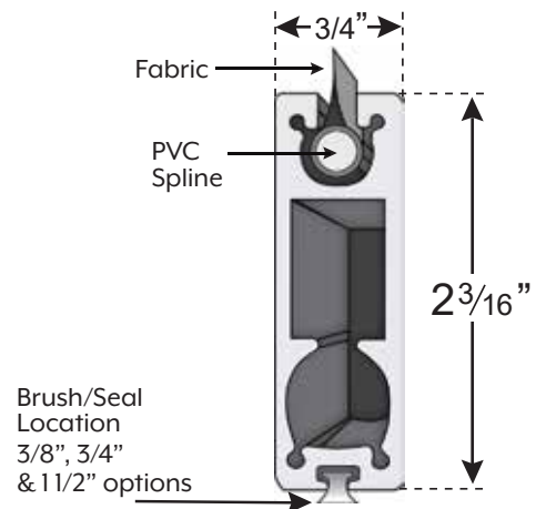
HD SCREEN • Hem Bar (Side View)
